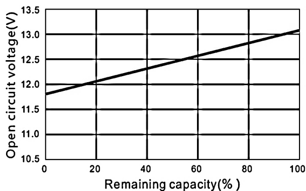
OCV vs Capacity
